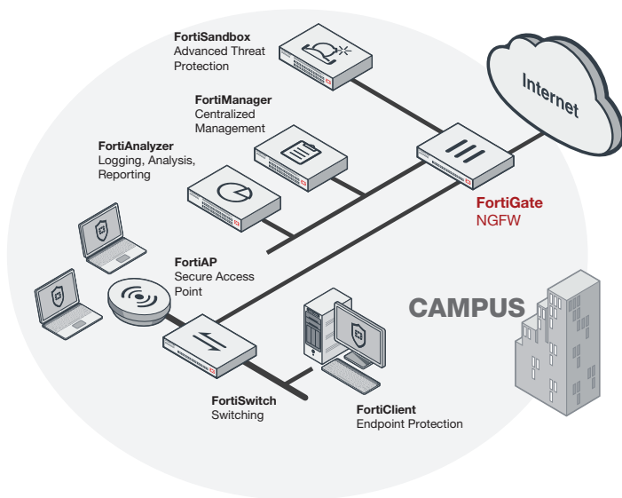
FortiGate 300D deployment in campus (NGFW)
